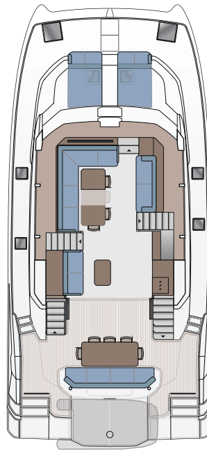
MAIN DECK GALLEY DOWN
