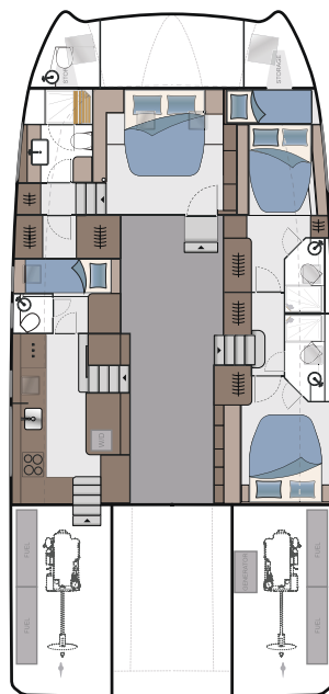
4-CABIN GALLEY DOWN
