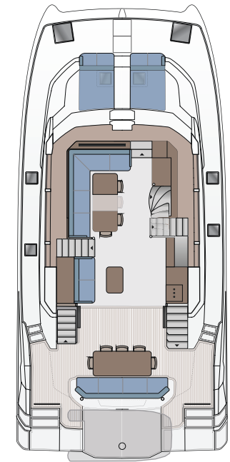
MAIN DECK GALLEY DOWN (SKYLounge FLYBRIDGE)
